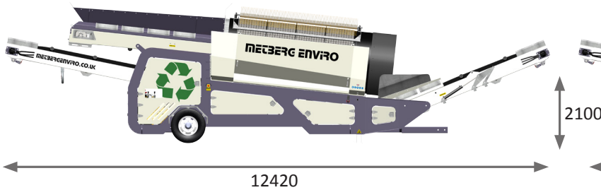
T3000 STOCKPILE WORKING DIMENSIONS
