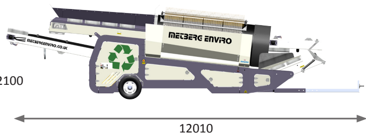
T3000 STOCKPILE TRANSPORT DIMENSIONS
