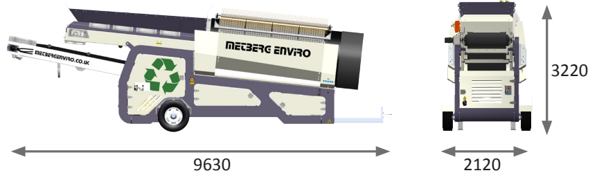
W3000/T3000 TRANSPORT DIMENSIONS
