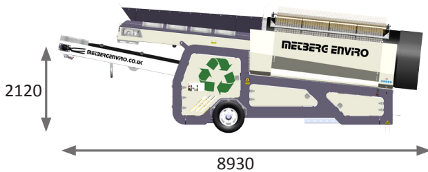
W3000/T3000 WORKING DIMENSIONS
