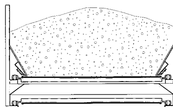
Samson® Body Section with Apron Belt and Parallel Entry
