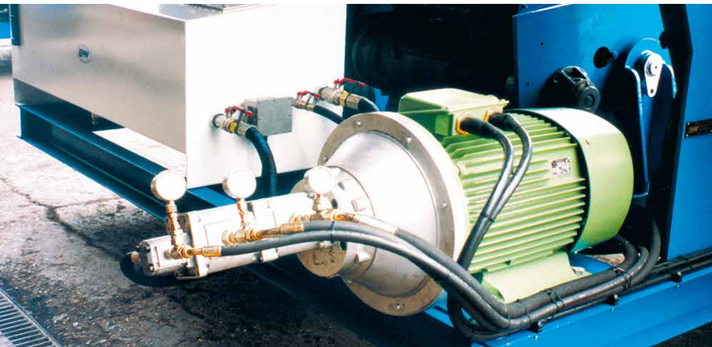
Electric Motor Drive with direct coupled triple section hydraulic pump and reservoir mounted beneath the Samson® section
