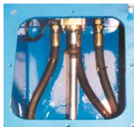
Rotary Potentiometer linked to the slew ring determines the wheel orientation and maintains both steering wheels in correct alignment using an electronic comparator system.
