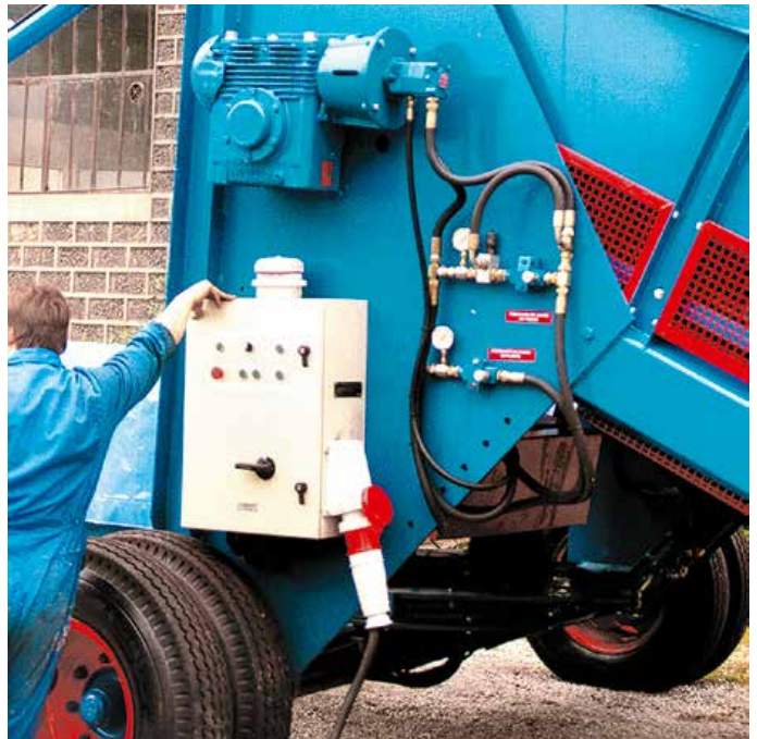
External control panel for electric motor drive with detachable cable
